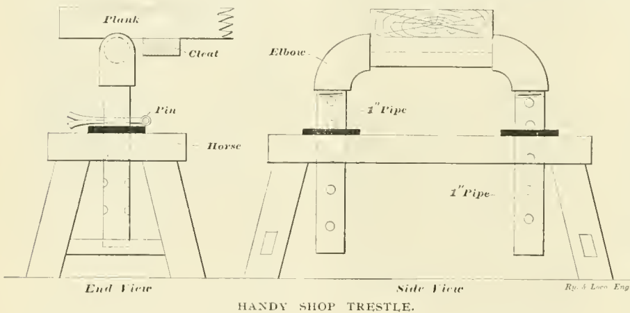
HANDY SHOP TRESTLE.
